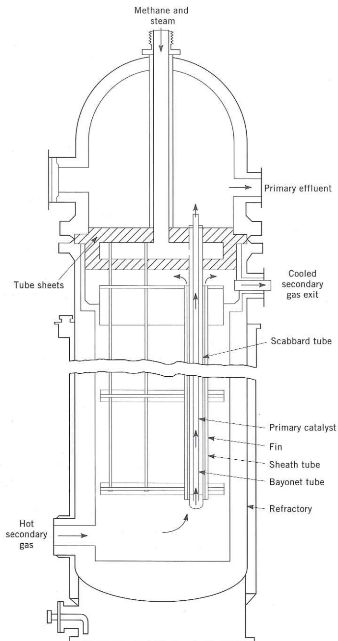
Fig. 3. ICI gas heated reformer (13).
