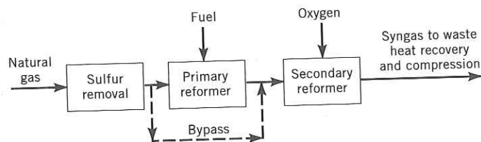
Fig. 2. Combined reforming.
