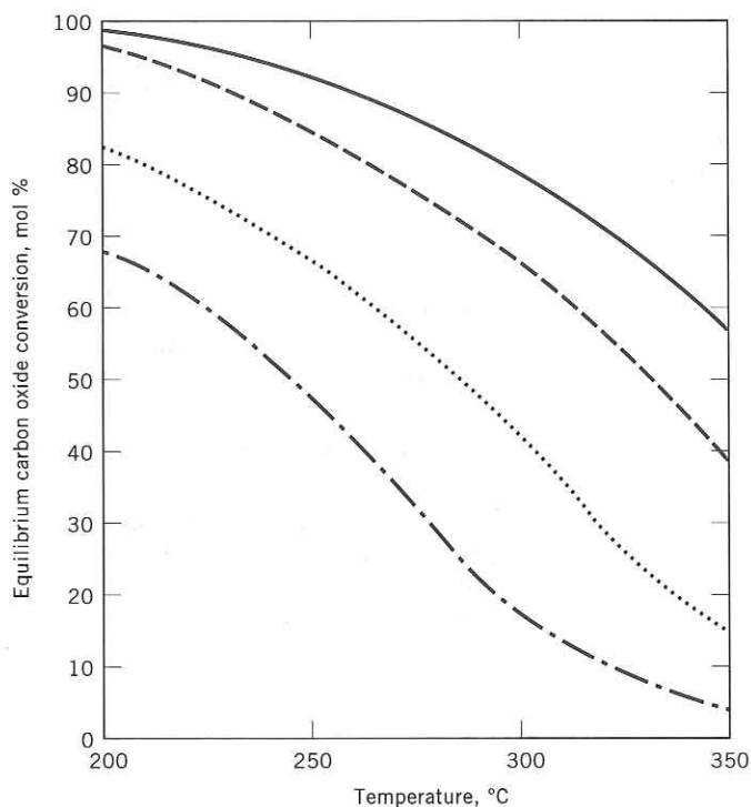
Fig. 1. Equilibrium conversion of carbon oxides to methanol based on reformed natural gas composition of 73% H_2 , 15% CO , 9% CO_2 , and 3% CH_4 where (—) is at 30 MPa, (---) is at 20 MPa, (····) is at 10 MPa, and (-·-·) is at 5 MPa. To convert MPa to atm, multiply by 9.87.
