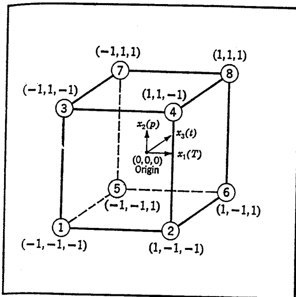
FACTORIAL DESIGN 2^3 in geometric form—Fig. 1
